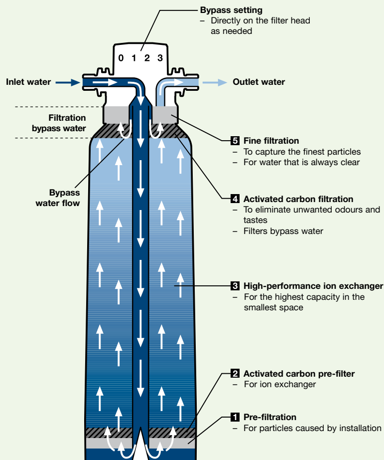
Configuration of a BWT bestclear filter cartridge with 5-way filtration
