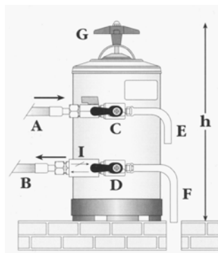
Fig 1: Installation Drawing
